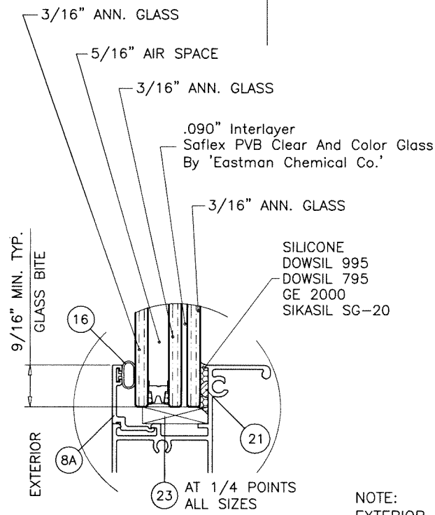
GLASS TYPE 'Ai' 15/16" OVERALL INSUL. LAM. GLASS
